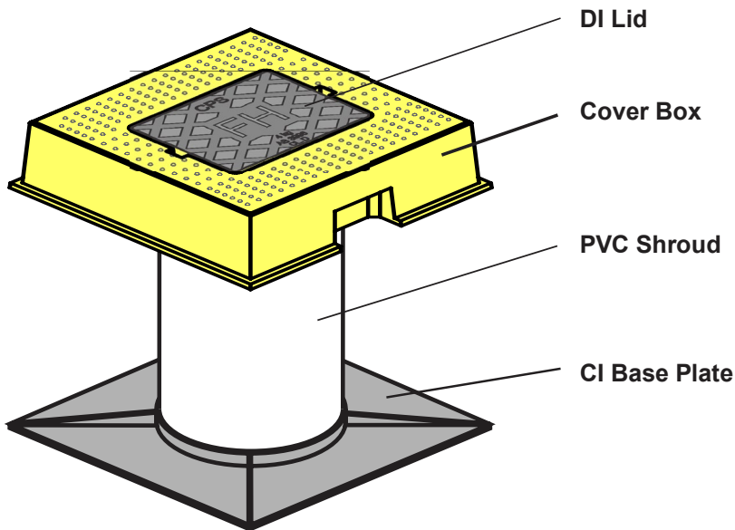
CLASS B COVER ASSEMBLY
