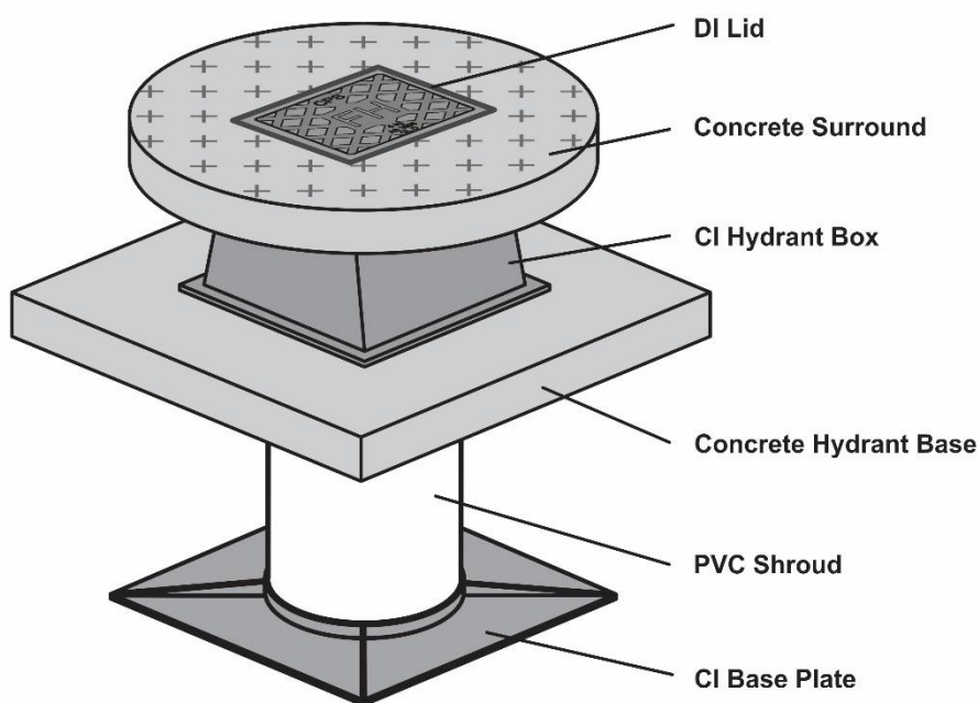
CLASS D COVER ASSEMBLY
