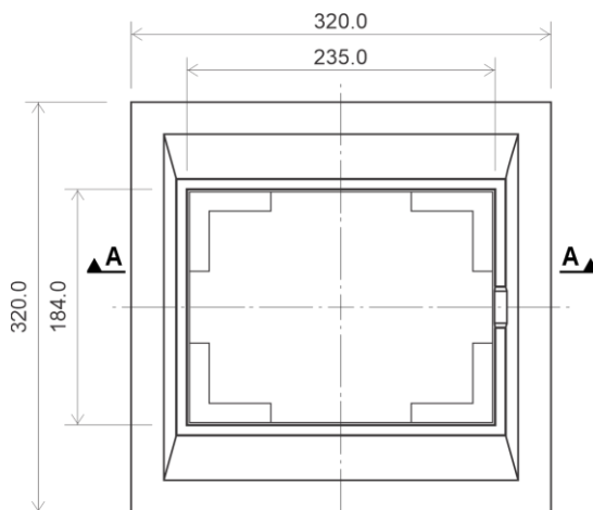
HYDRANT BOX – TOP VIEW
