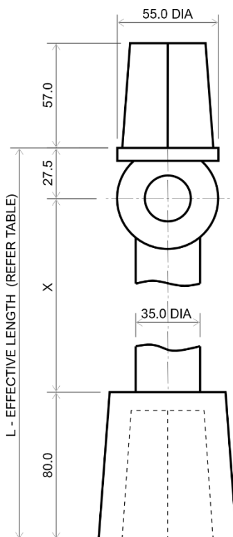
EXTENSION SPINDLE
